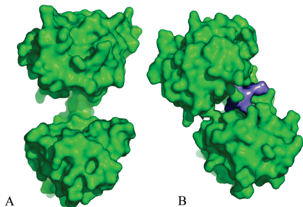
FIGURE 4: Domain closure upon ligand binding. (A) Surface representation of human apo U3S, which adopts the most open conformation observed in the various crystal structures. (B) Product bound T. thermophilus U3S showing how the domains close around the uro'gen ligand (purple). Both panels are in the same orientation as Figure 2.
