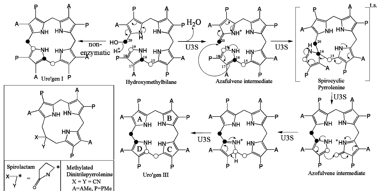
FIGURE 1: The proposed mechanism of U3S catalyzed formation of uro'gen III (3). This figure resembles that of Roessner et al. (33). Spirolactam, a transition state mimic, has been shown to be a competitive inhibitor of U3S (36), and the structure of a synthetic precursor, methylated dinitrilepyrrolenine, has been determined (6). A = CH 2 CO 2 , P = CH 2 CH 2 CO 2 .
